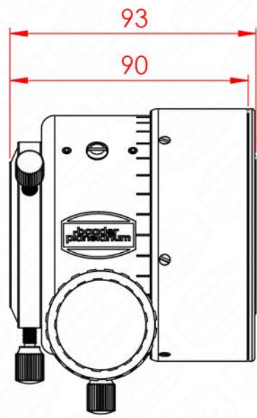
measurements with and without 3.3"/2" reducer
